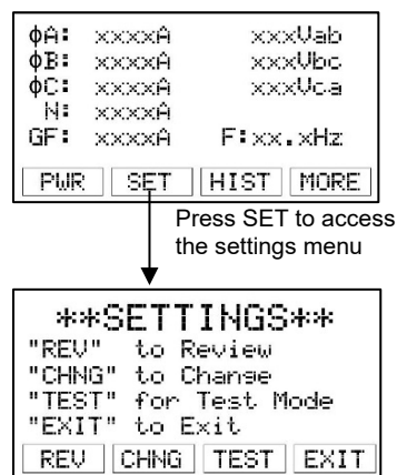
Figure D: Settings Menu first screen
