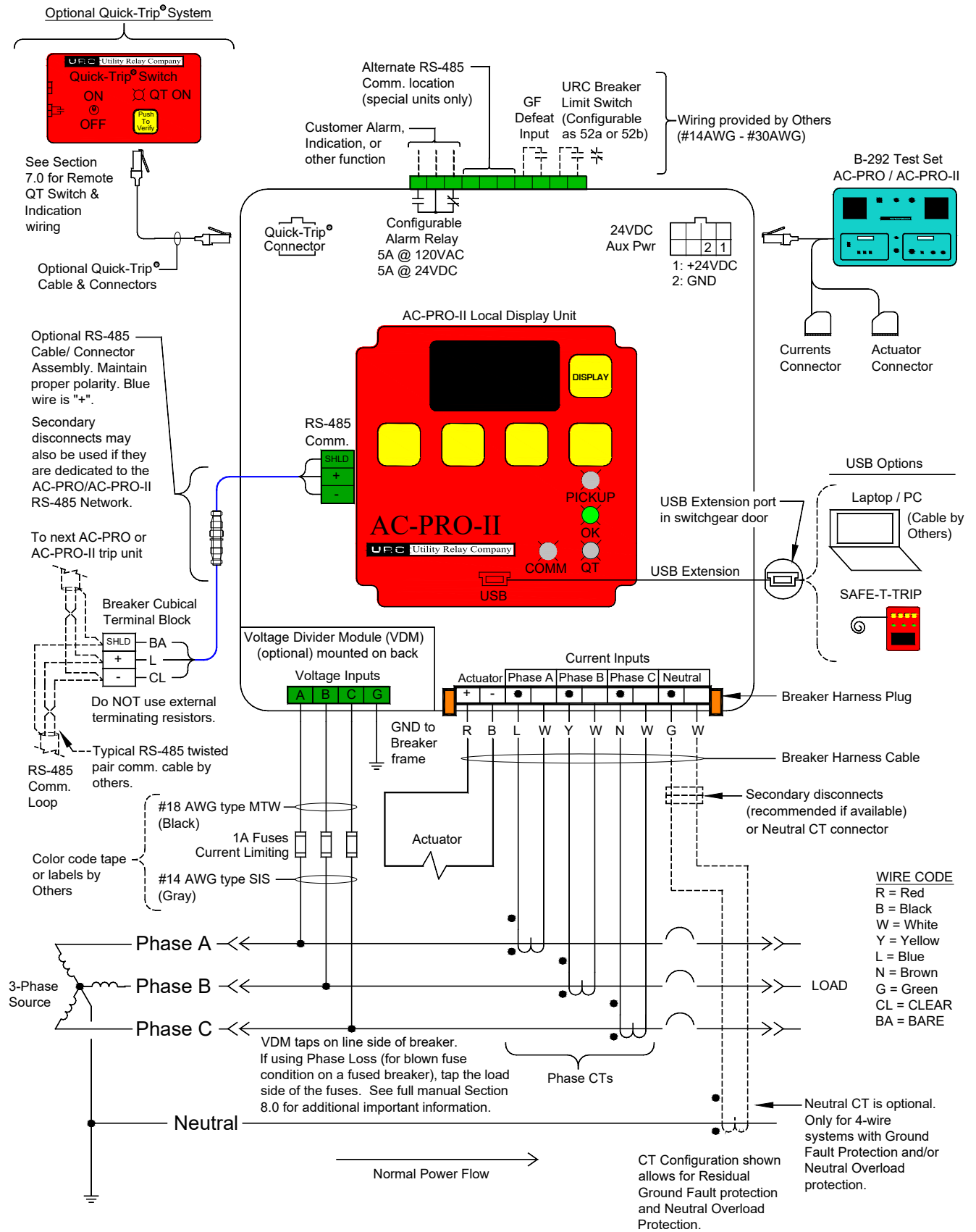
Figure E: AC-PRO-II Typical Wiring Diagram
