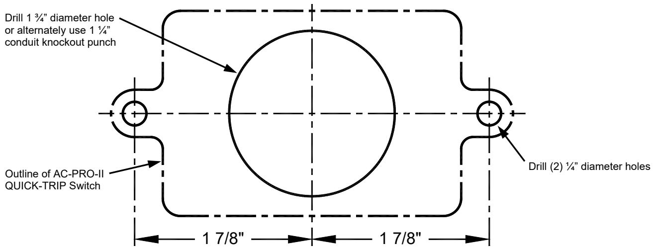
Figure H: AC-PRO-II QUICK-TRIP Switch Drilling Plan
