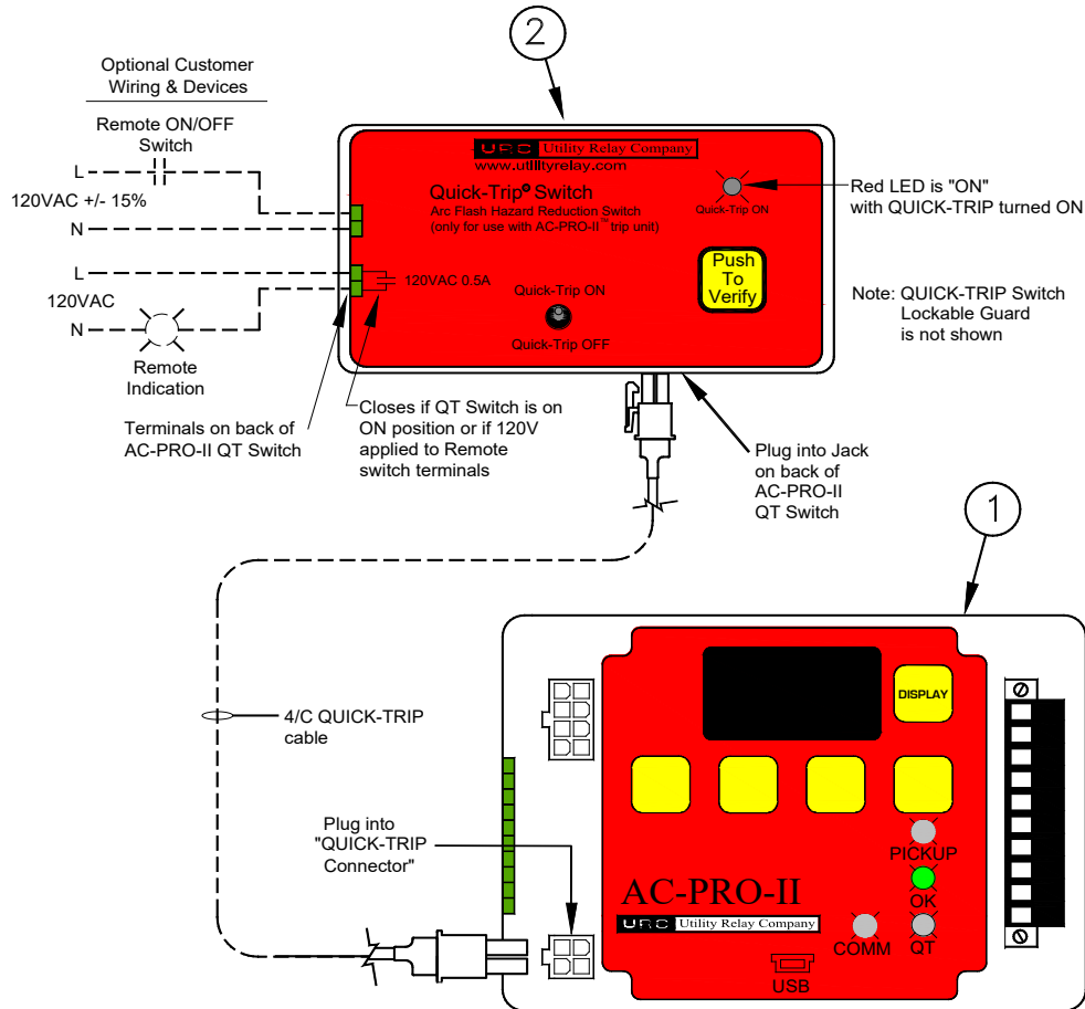
Figure G: QUICK-TRIP System and Connections (Option 1)
