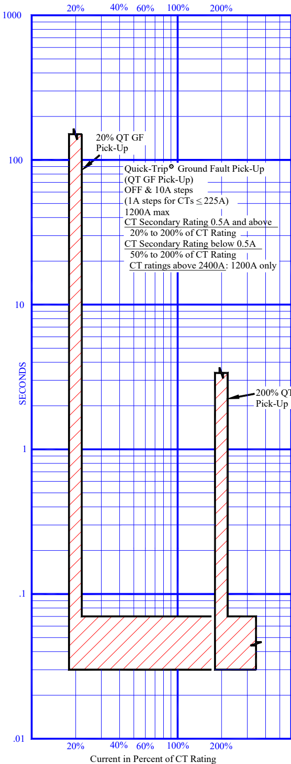
Quick-Trip® Ground Fault Time Current Curve
